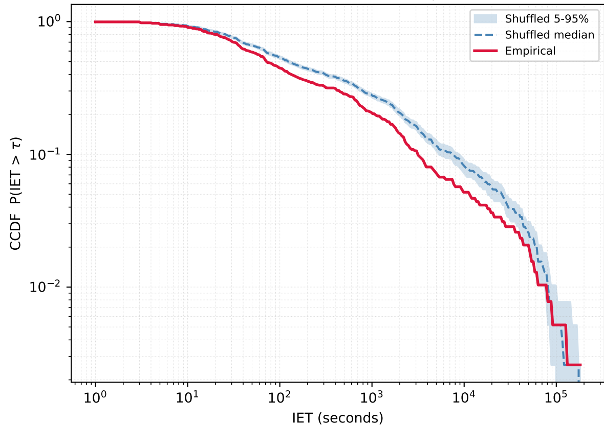
User 1505404600 - Empirical vs Reshuffled | KS=0.095 p=0.000
